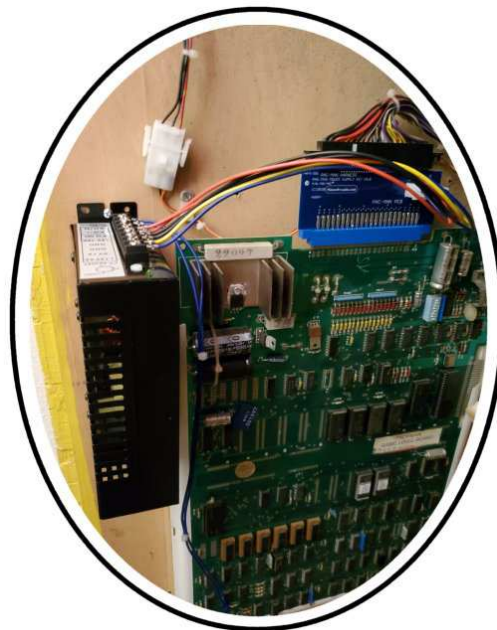
Power Supply Installed
