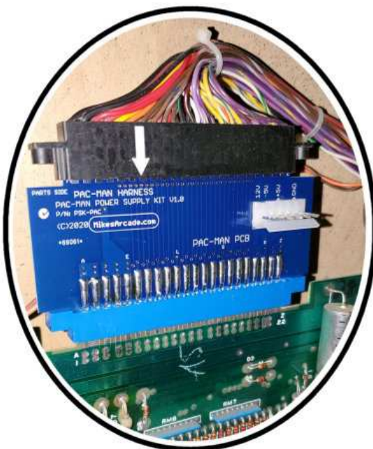
Installation Stack
