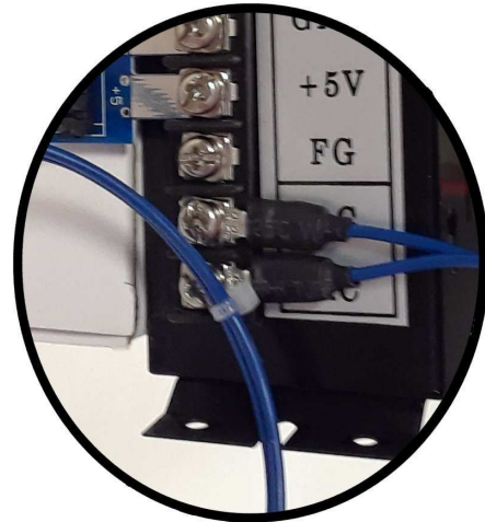
Attach the blue spades to the two A/C lugs of the new switching power supply.
