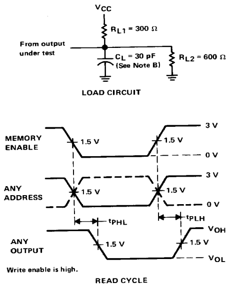
FIGURE 1—SWITCHING CHARACTERISTICS
