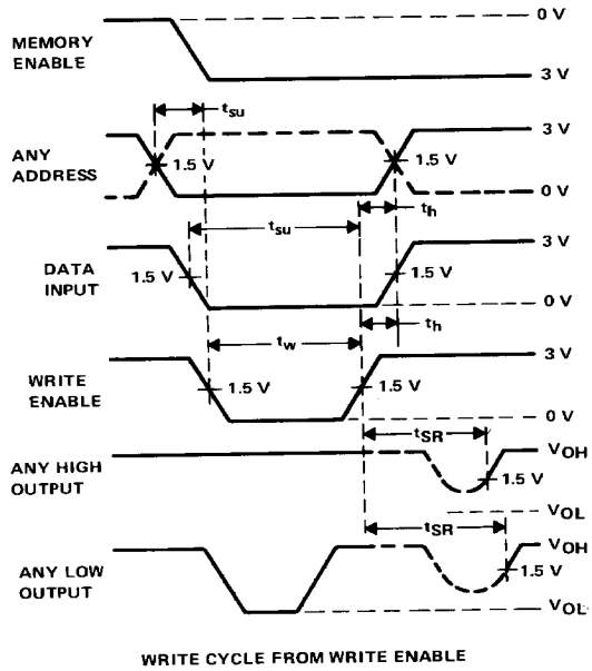
FIGURE 1—SWITCHING CHARACTERISTICS
